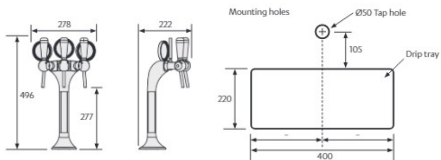
HC50 3 Spout tap with badge
